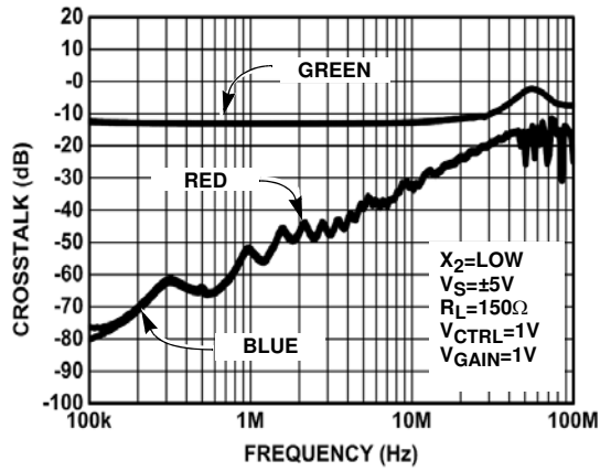
FIGURE 18. GREEN CROSSTALK (CABLE LENGTH = 600ft.)
