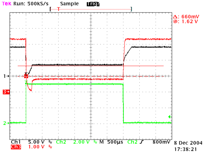
FIGURE 18. WOC OPERATION
