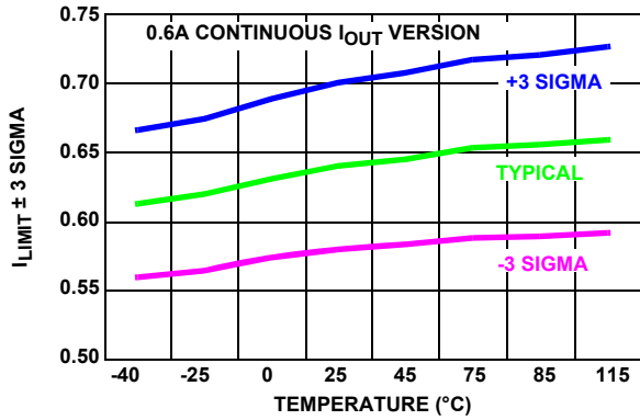
FIGURE 9. LIMITING CURRENT \pm 3 SIGMA, V_{IN} = 5V
