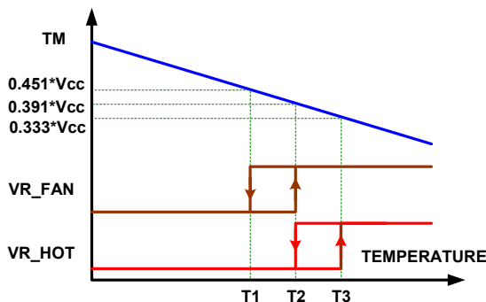
FIGURE 19. VR_HOT AND VR_FAN SIGNAL vs TM VOLTAGE Based on the NTC temperature characteristics and the desired threshold of the VR_HOT signal, the pull-up resistor R_{TM1} of TM
