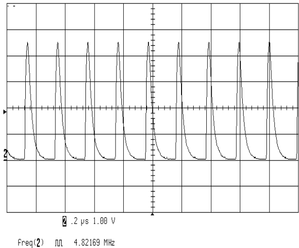
FIGURE 18. SYNC WAVEFORM
