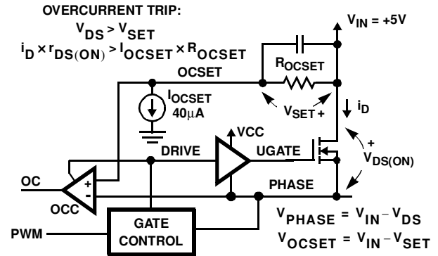
FIGURE 2. OVERCURRENT DETECTION
