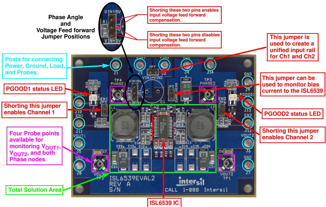
FIGURE 1. ISL6539EVAL1 BOARD
