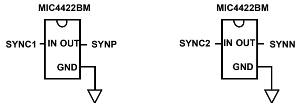
FIGURE 26B. NONINVERTING DRIVERS
