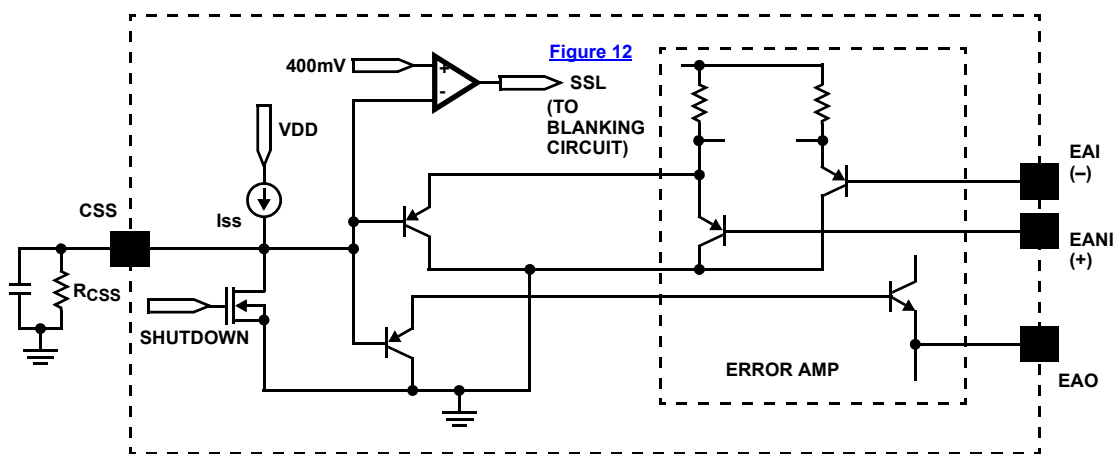
FIGURE 7. SIMPLIFIED CLAMP/SOFT-START
