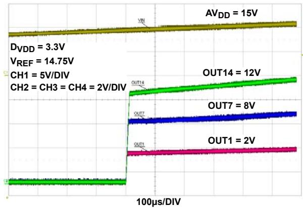
FIGURE 22. OUT1-OUT7-OUT14 AT POWER-ON (ZOOMED IN)
