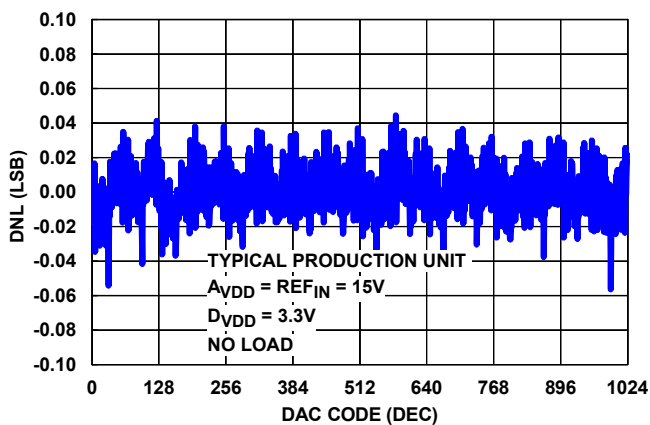
FIGURE 18. DAC1-DAC15 TYPICAL DNL ( \text{REF}_{\text{IN}} = \text{A}_{\text{VDD}} = 15\text{V} ) AT -40^\circ\text{C}
