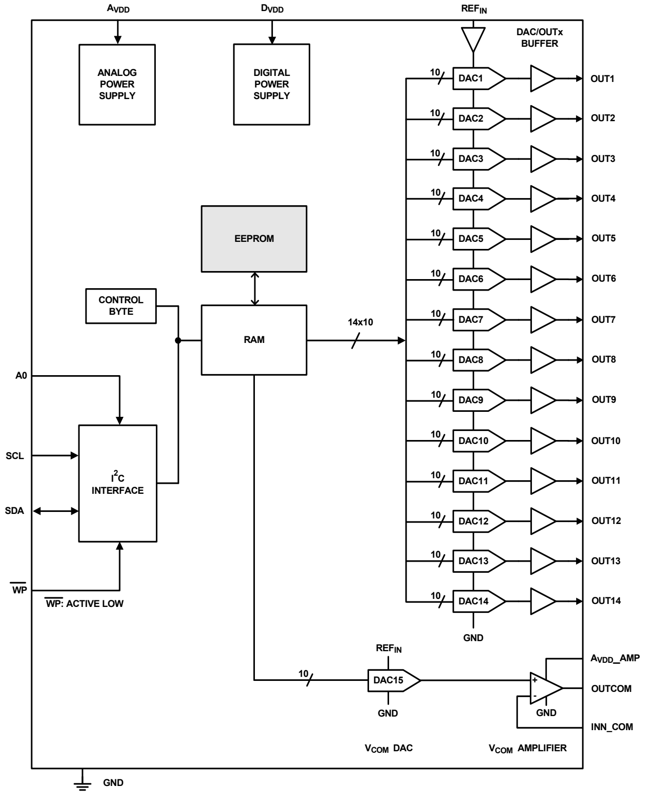
FIGURE 2. BLOCK DIAGRAM
