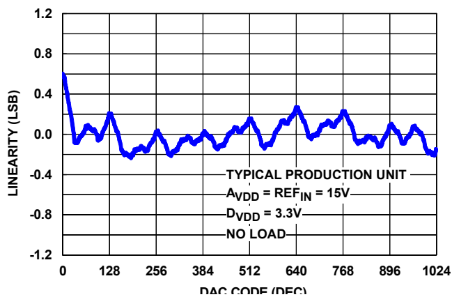
FIGURE 19. DAC1-DAC15 INL ( \text{REF}_{\text{IN}} = \text{A}_{\text{VDD}} = 15\text{V} ) AT +105^\circ\text{C}
