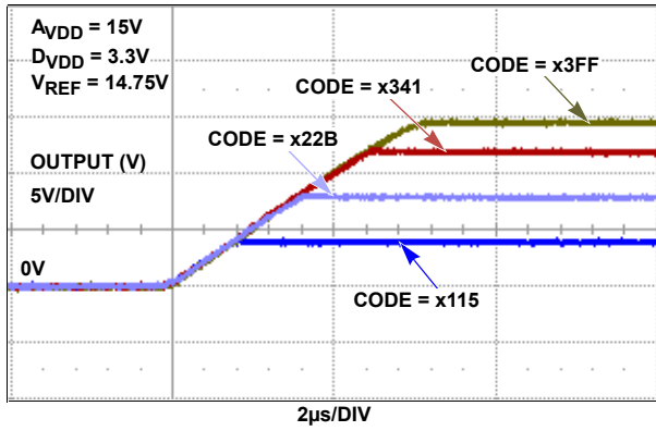
FIGURE 9. OUT1-OUT14 POSITIVE SLEW RATE (DAC CODE CHANGE)
