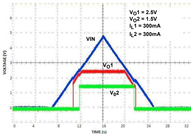
FIGURE 11. POWER-UP/POWER-DOWN
