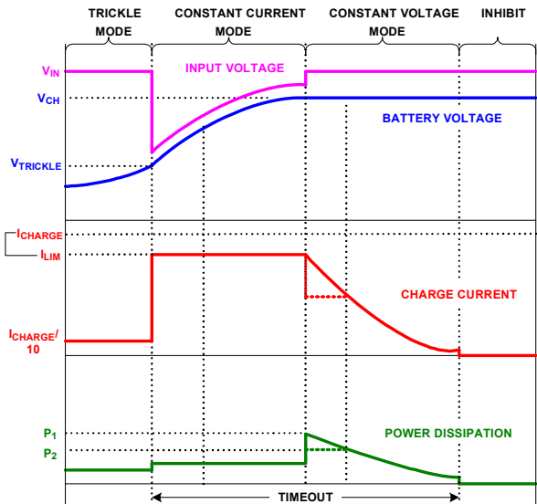
FIGURE 20. TYPICAL CHARGE CURVES USING A CURRENT-LIMITED ADAPTER
