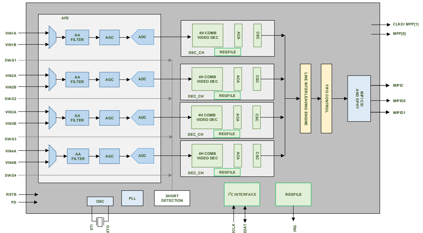
FIGURE 1. ISL79985 BLOCK DIAGRAM
