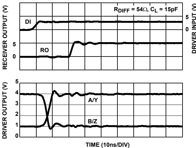
FIGURE 13. DRIVER AND RECEIVER WAVEFORMS, LOW TO HIGH
