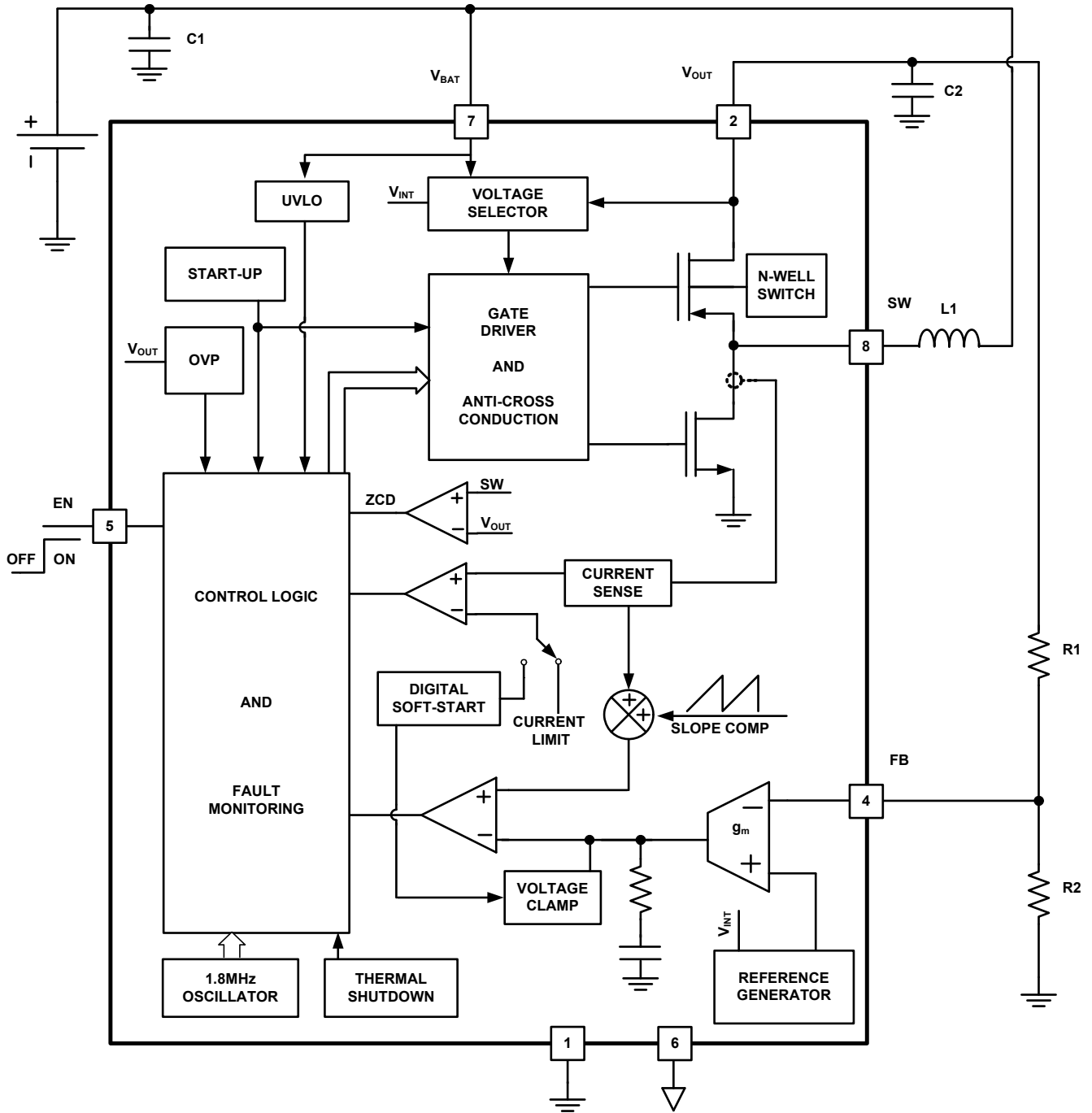
FIGURE 3. BLOCK DIAGRAM
