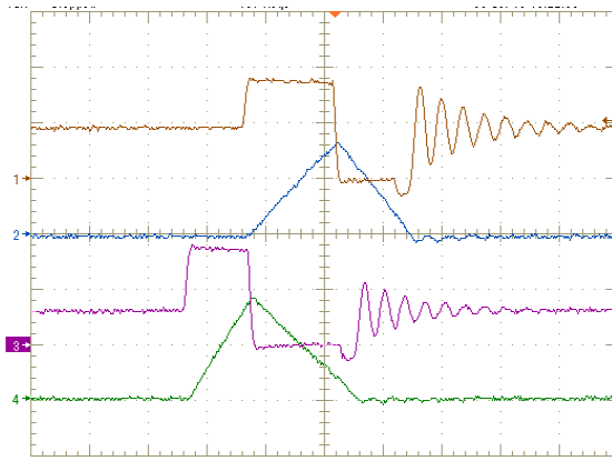
FIGURE 10. INDUCTOR CURRENT RIPPLE ( V_{IN} = 3.6V , PFM, TIME SCALE = 200ns) CH1: SW1 (2V/DIV), CH2: IL1 (200mA/DIV), CH3: SW2 (2V/DIV), CH4: IL2 (200mA/DIV)
