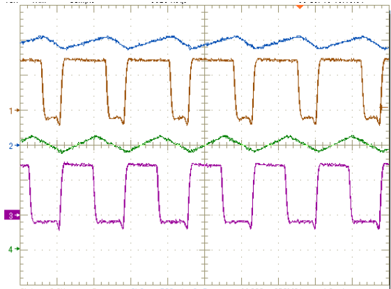
FIGURE 11. INDUCTOR CURRENT RIPPLE ( V_{IN} = 3.6V , FULL LOADING, PWM, TIME SCALE = 200ns) CH1: SW1 (2V/DIV), CH2: IL1 (500mA/DIV), CH3: SW2 (2V/DIV), CH4: IL2 (500mA/DIV)
