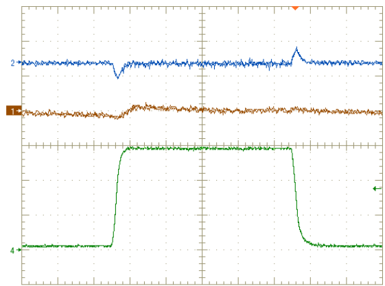
FIGURE 13. DCD2 TRANSIENT RESPONSE ( V_{IN} = 3.6V , STEP LOAD: 150mA TO 1500mA) CH1: VODCD1 (100mV/DIV, AC), CH2: VODCD2 (50mV/DIV, AC), CH4: IL4 (500mA/DIV)
