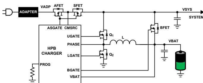
FIGURE 1. HPB CHARGER CONFIGURATION
