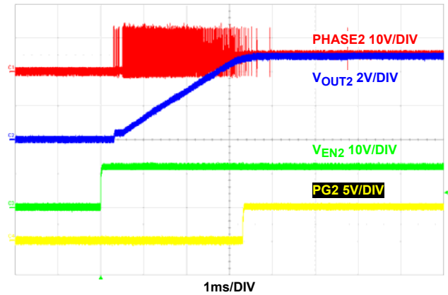
FIGURE 13. CH2 START-UP AT NO LOAD (PFM)
