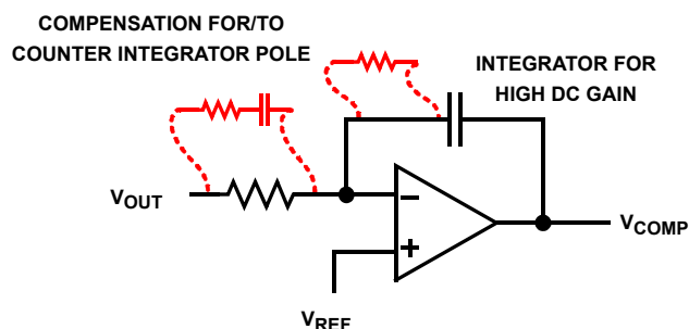
FIGURE 62. INTEGRATOR ERROR-AMPLIFIER CONFIGURATION
