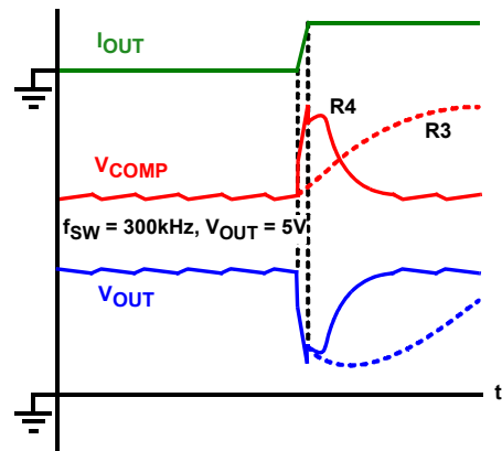
FIGURE 2. R3™ vs R4™ IDEALIZED TRANSIENT RESPONSE
