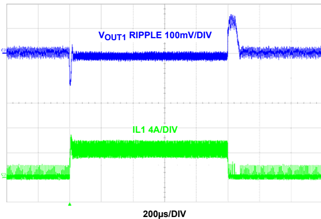
FIGURE 50. CH1 LOAD TRANSIENT (PFM)
