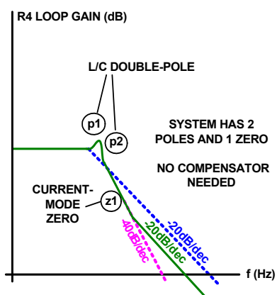
FIGURE 65. UNCOMPENSATED R4™ OPEN-LOOP RESPONSE
