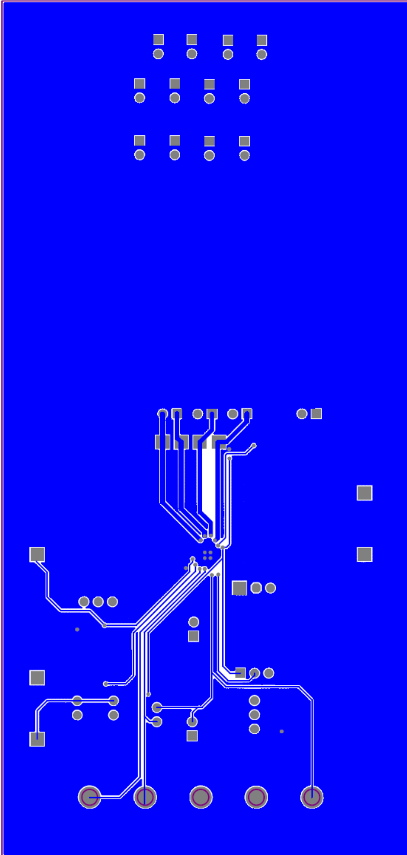
FIGURE 3. BOTTOM LAYER
