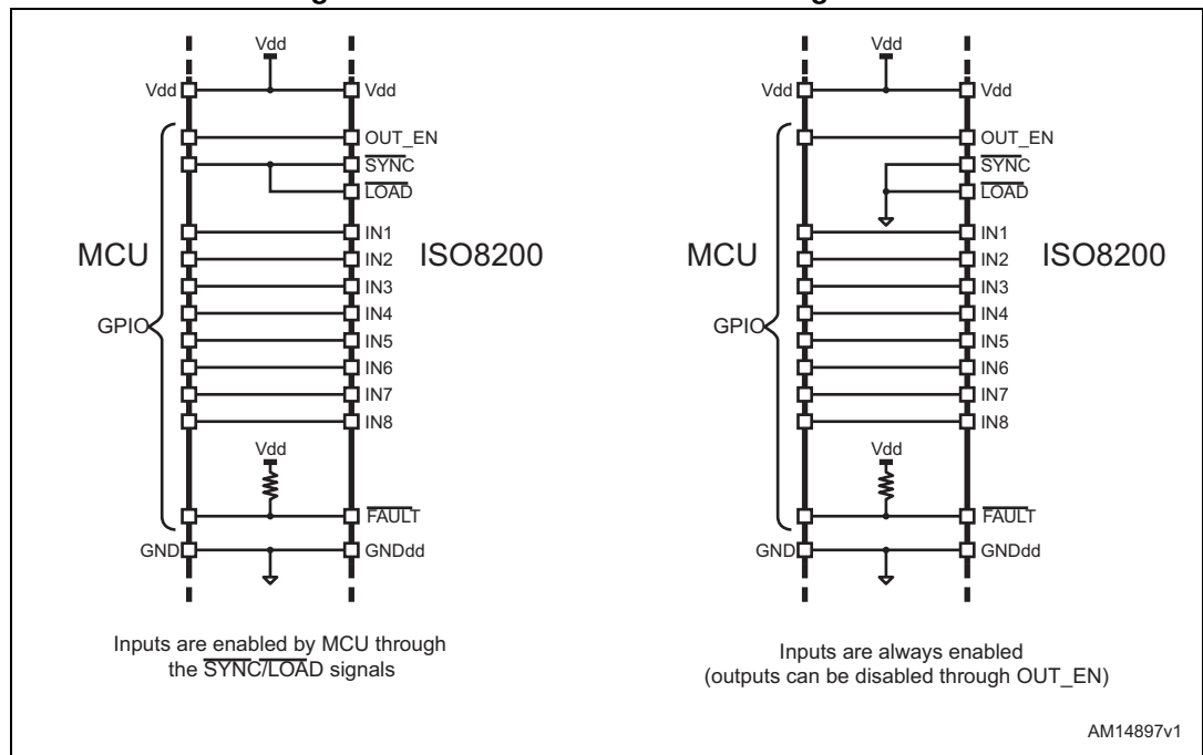
Figure 9. Direct control mode IC configuration
