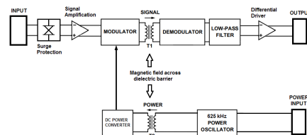
IsoBlock Q single channel block diagram.
