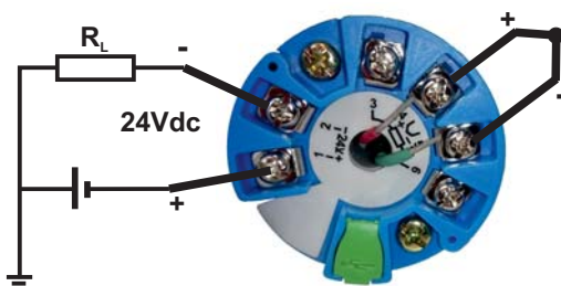
THERMOCOUPLE
