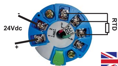
RTD 3-WIRE
