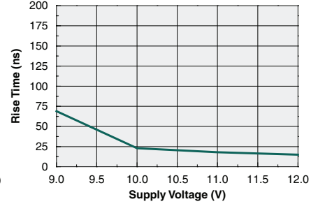
Turn-On Rise Time vs. Supply Voltage
