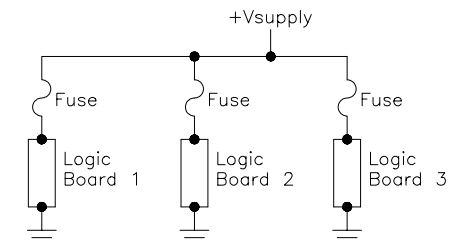
Fig. 9. Normal fusing links in series with each board
