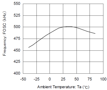
(8) Oscillation Frequency Temperature Characteristics
