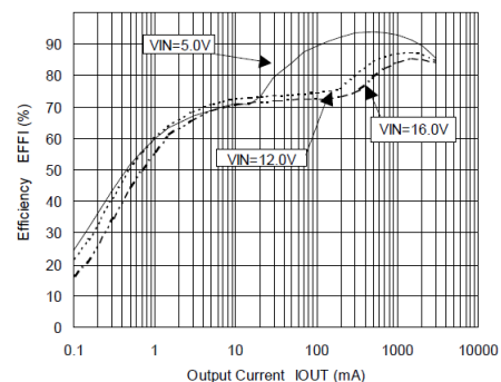
IXD3221A095MR - V OUT = 3.3 V, f OSC = 500 kHz, C IN = C L = 47 μF (OS-Con), L = 10 μH (CDRH8D43, (SUMIDA), Q - CPH3308, C FB = 1.0 μF (ceramic), R FB = 10Ω
