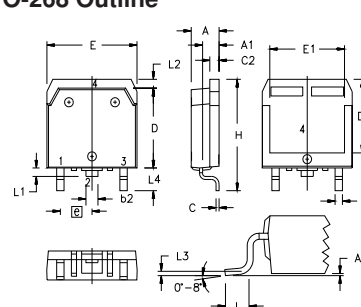
TO-268 Outline
