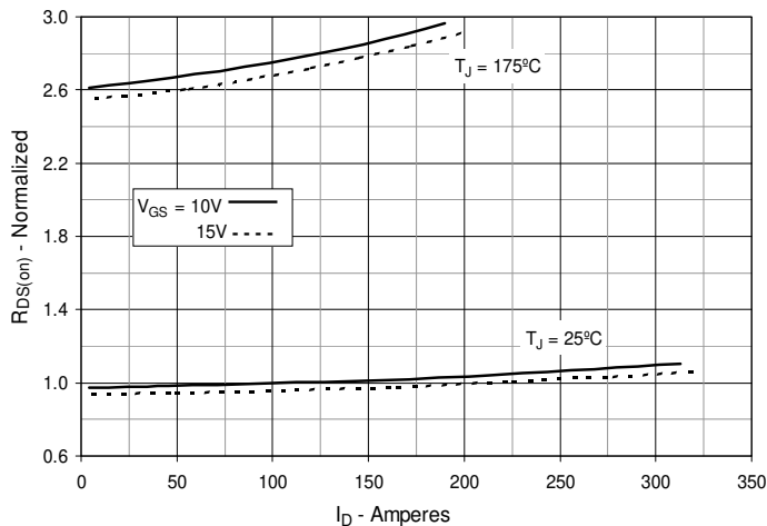
Fig. 5. R_{DS(on)} Normalized to I_D = 105\text{A} Value vs. Drain Current
