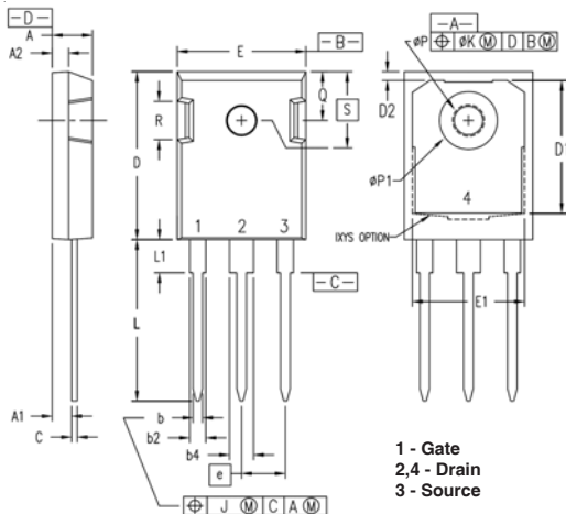
TO-247 Outline
