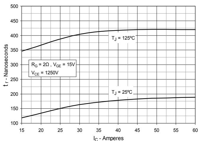
Fig. 13. Resistive Turn-on Rise Time vs. Drain Current
