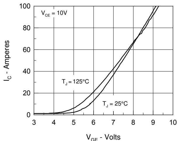
Fig. 5. Admittance Curves
