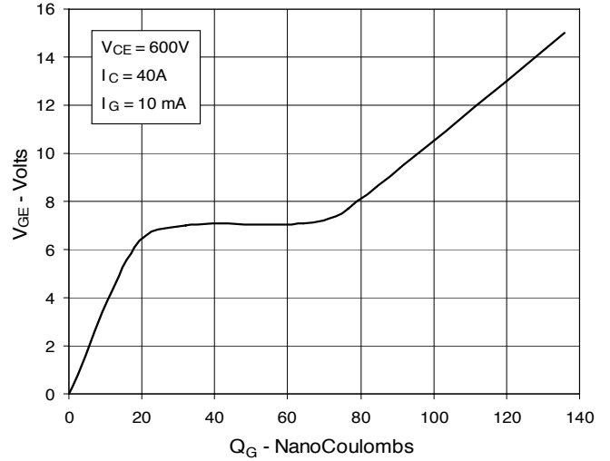
Fig. 14. Gate Charge
