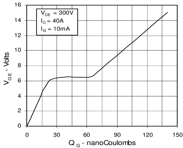
Fig. 15. Gate Charge
