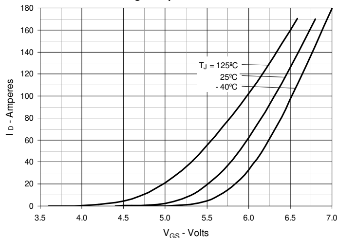
Fig. 8. Input Admittance
