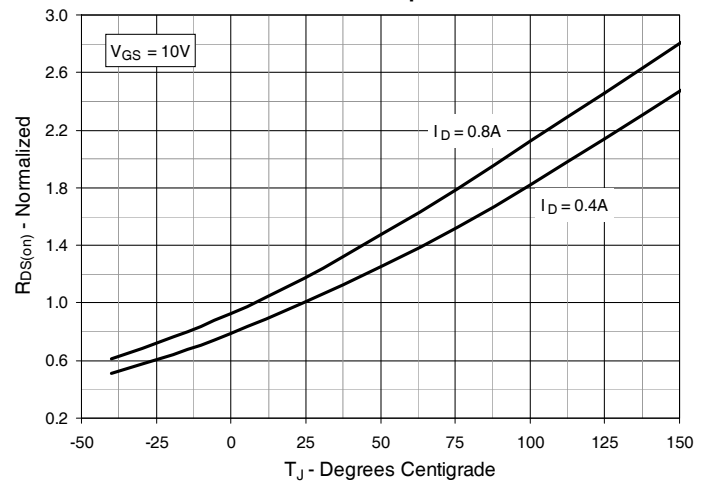
Fig. 4. R_{DS(on)} Normalized to I_D = 0.4\text{A} Value vs. Junction Temperature
