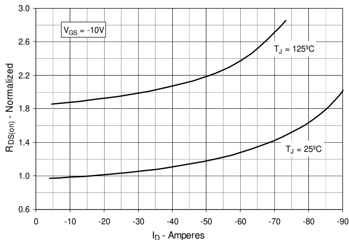
Fig. 5. R_{DS(on)} Normalized to I_D = -18A Value vs. Drain Current
