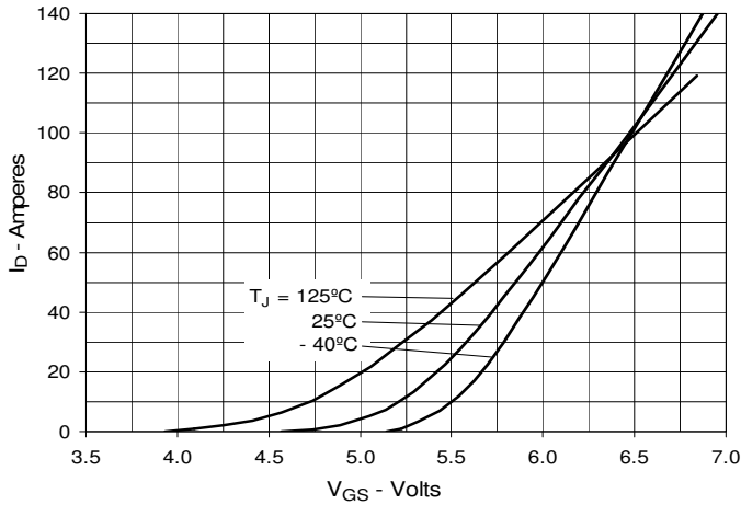
Fig. 7. Input Admittance
