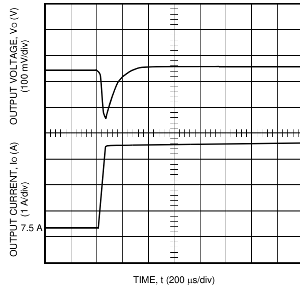
Figure 7. Typical JAW075A Transient Response to Step Increase in Load from 50% to 75% of Full Load at Room Temperature and 48 Vdc Input (Waveform Averaged to Eliminate Ripple Component.)
