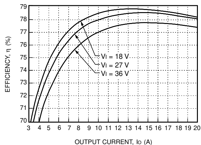
Figure 8. Typical JC100F Converter Efficiency vs. Output Current at Room Temperature
