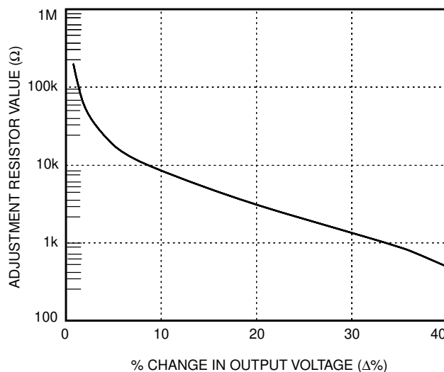
Figure 19. Resistor Selection for Decreased Output Voltage
