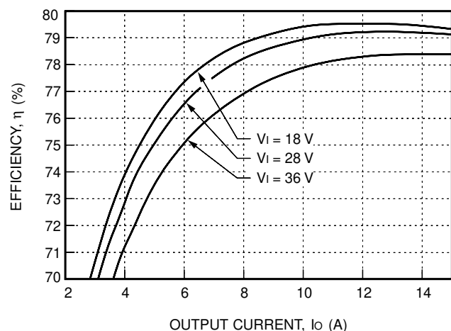
Figure 7. Typical JC075F Converter Efficiency vs. Output Current at Room Temperature
