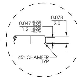
TIP DETAIL FOR GTT-11
