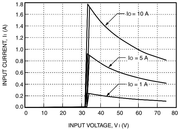
Figure 1. Typical JFW050A Input Characteristics at Room Temperature
