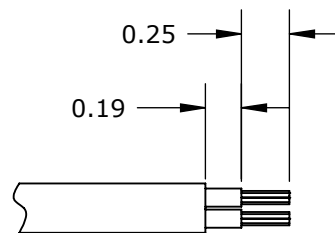
RECOMMENDED STRIPPING LENGTH
