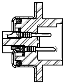
Rear side (cross section)
