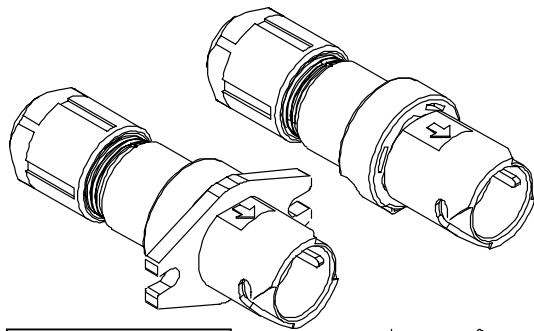
Wall Mounting Receptacle
