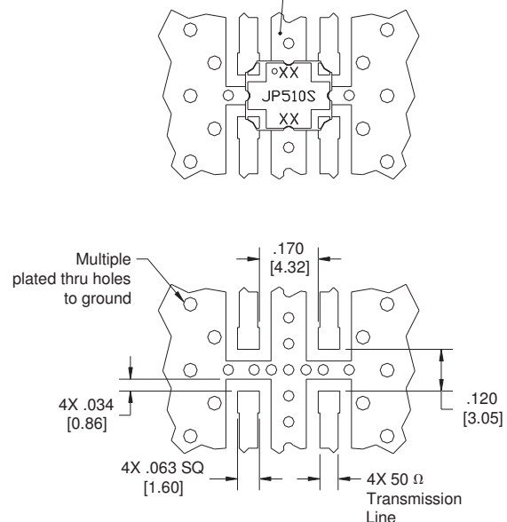
Dimensions are in Inches [Millimeters] JP510S Mounting Footprint
