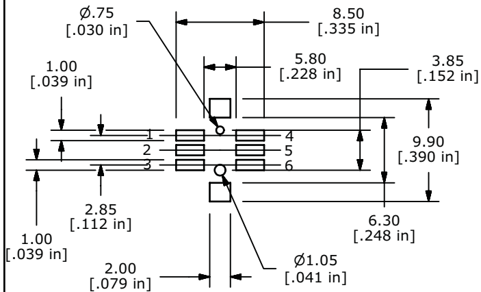
SOLDER LAYOUT
