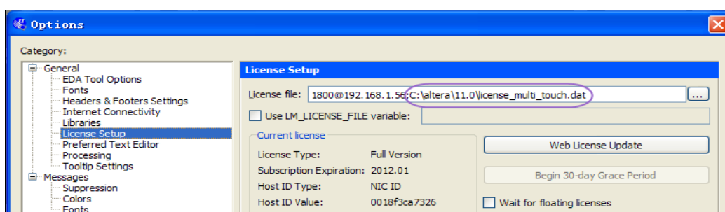
Figure 1-2 License Setup
