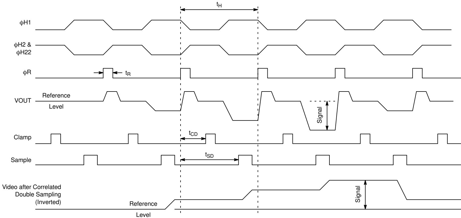
Figure 12. Pixel Timing - 1x1
