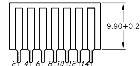
BACK VIEW
