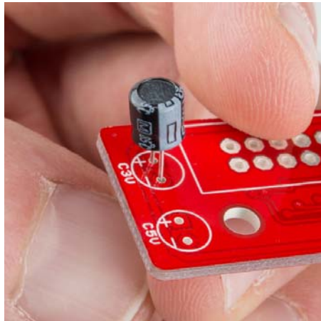
Capacitor Polarity
