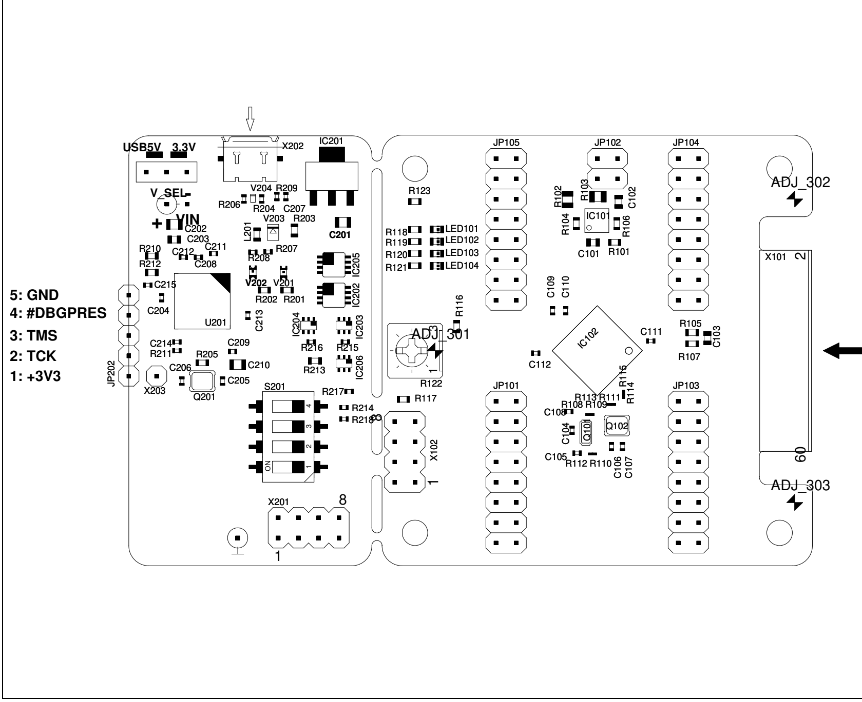
Figure 15 CR number of XMC1400 Boot Kit
