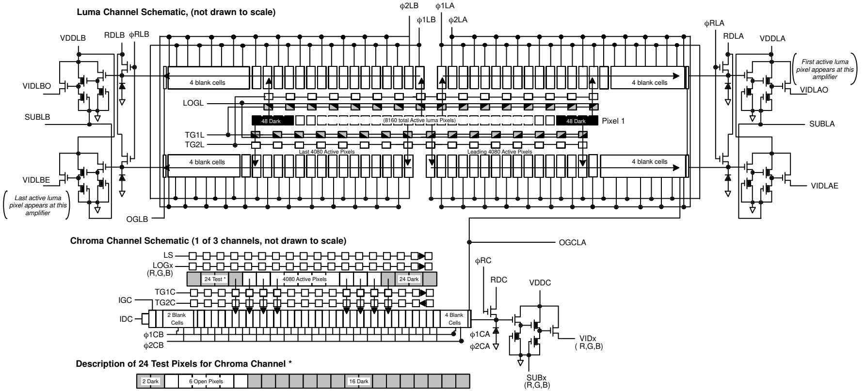
Figure 6. Device Schematic
