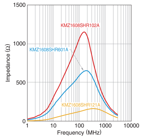
KMZ1608SHR series
