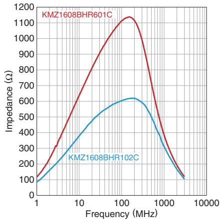
KMZ1608BHR series
